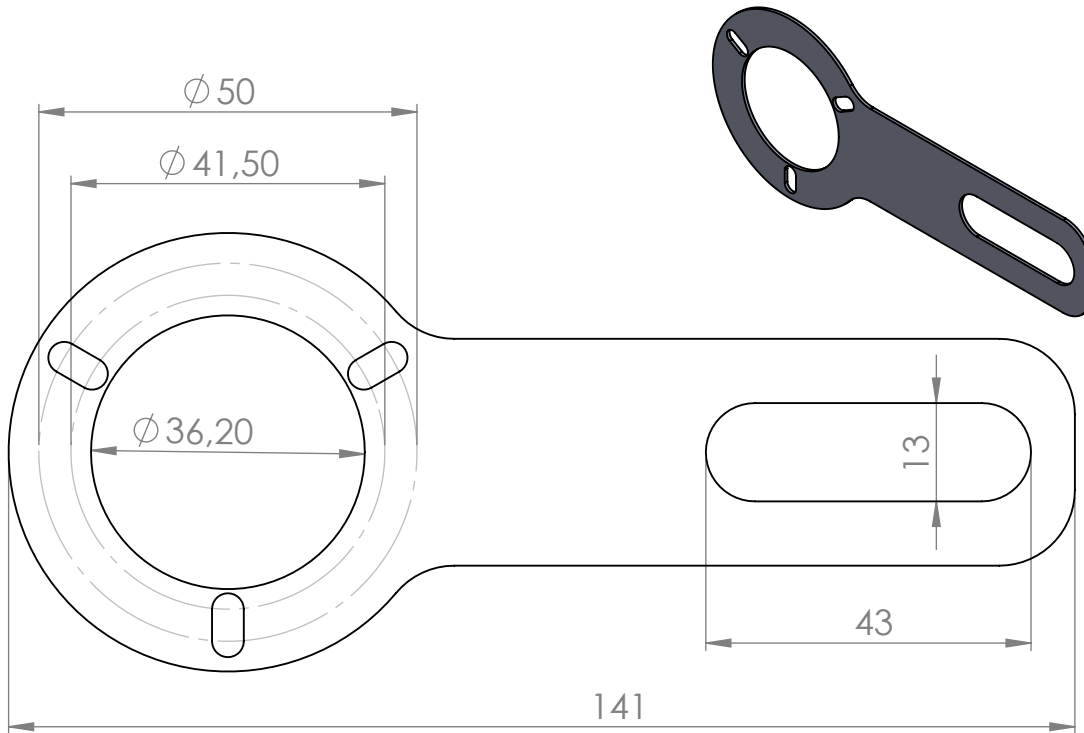
3-210-2151 Rotationstop - torsion spring
