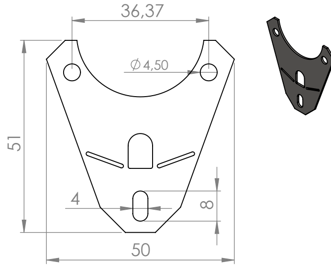
3-213-1733 Rotationstop
