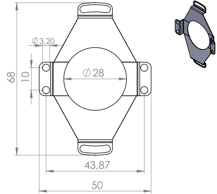
3-221-1121 Stator coupling
