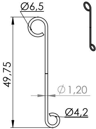
3-210-2151 Rotationstop - torsion spring
