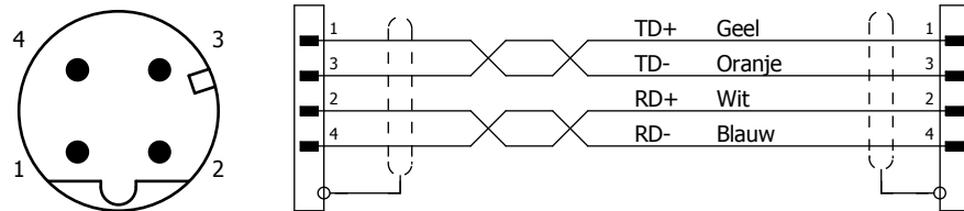
KBL846-xxx 4P M12 male D-Gecodeerd
