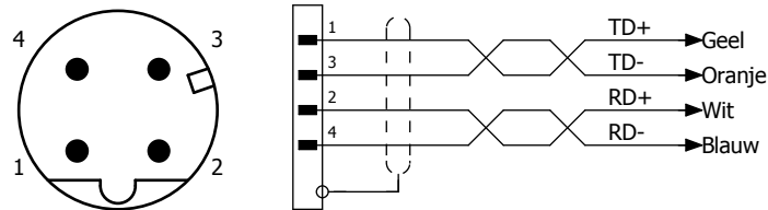
KBL844-xxx 4P M12 male D-Gecodeerd
