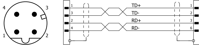
KBL840-xxx 4P M12 male D-Gecodeerd
