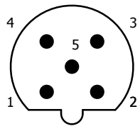
KBL030-xxx 5P M12 male B-Gecodeerd
